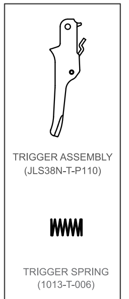
JLS38N-T-SQ2 SEQUENTIAL TRIGGER SET (FOR MODEL JLS38N, JLS38S)
