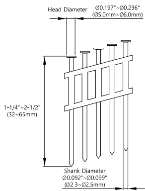
15° Degree Flat Plastic sheet Collated Nails
