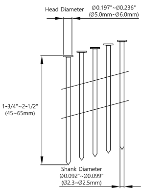
15° Degree Flat Wire Welded Nails
